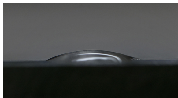
Figure 4. High-energy surface (liquid spreads out, indicating good adhesion)
