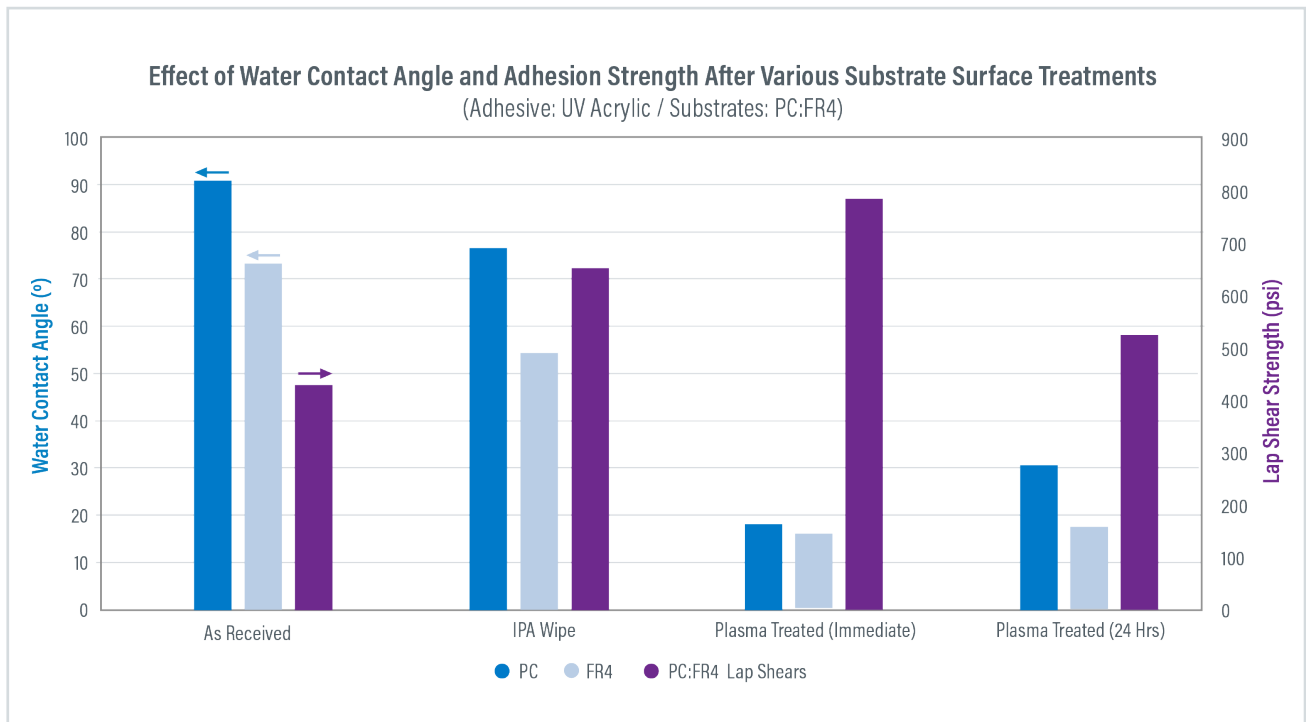
Graph 5. Contact angle (left) and adhesion strength (right) for PC to FR-4 (UV-curable acrylate)
