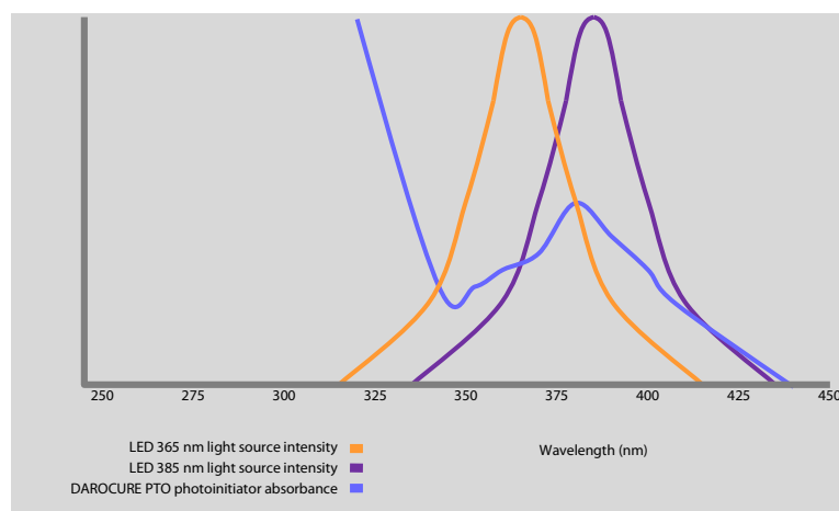
Figure 2. Photoinitiator absorption compared to 365 nm and 385 nm LED curing-light spectral distributions.
