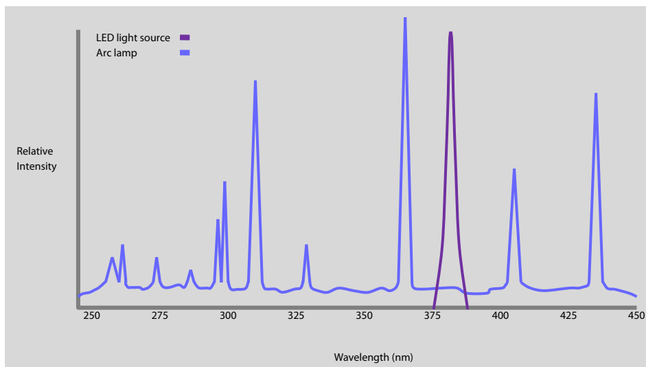
Figure 2. Wavelength distribution of an arc lamp and LED light source in the visible-light range
