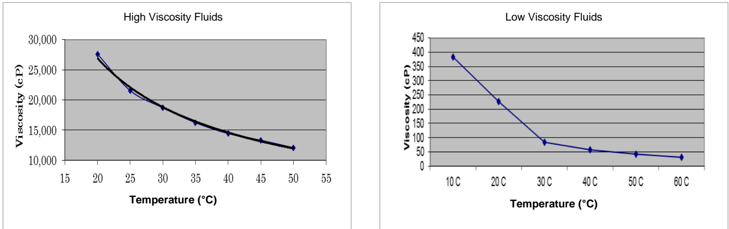
Figure 1. Temperature vs. Viscosity for High & Low Viscosity Materials
