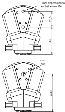
Fig.: Mounting
